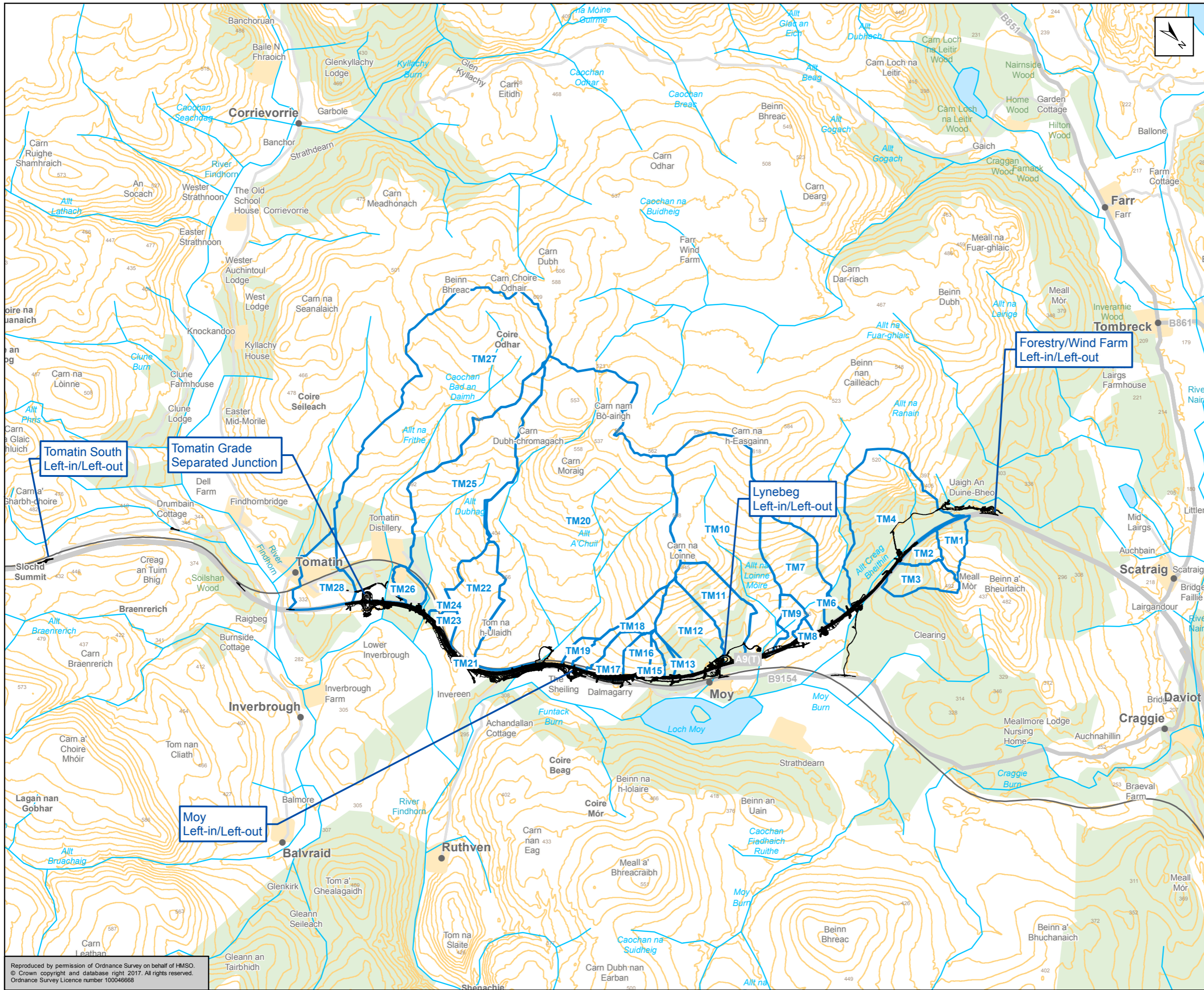
Figure A.11.2.6 Watercourse Catchment Plan
