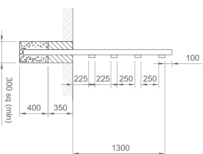
SECTION THROUGH CENTERLINE OF MAIN POSTS
