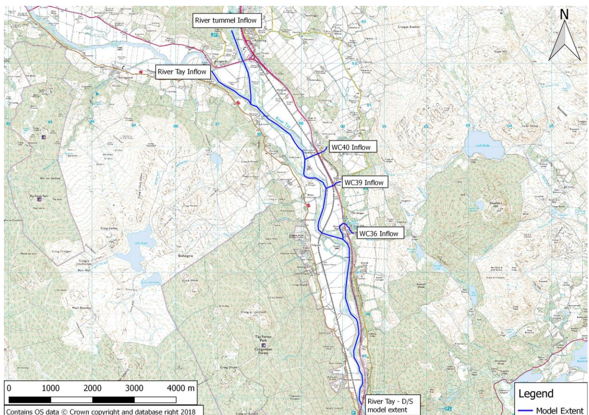
Diagram 3: Model III extents together with flow estimation locations
