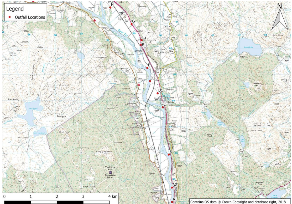
Diagram 8: Location of the proposed outfalls
