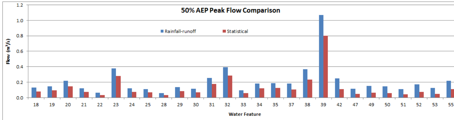
Diagram 1: Comparison of the 50% AEP (2-year) peak flow estimates from the FEH Rainfall-runoff and the FEH Statistical methods for catchments <25km2
