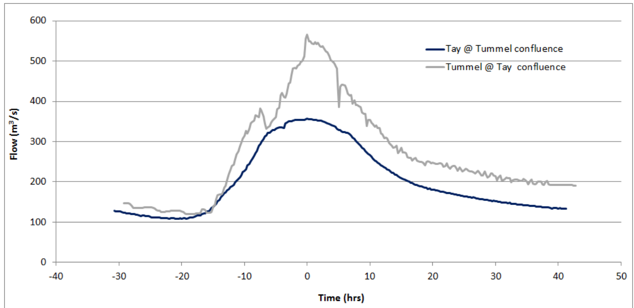
Diagram 7: Model III inflow hydrographs for Run 2 (Rivers Tay and Tummel: 50% AEP (2-year))
