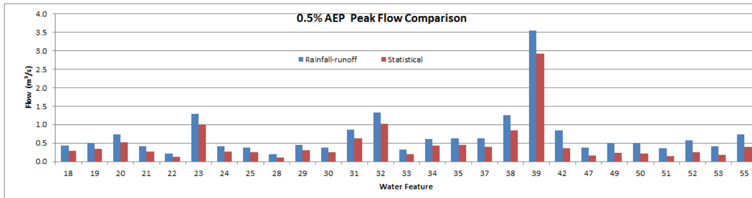
Diagram 2: Comparison of the 0.5% AEP (200-year) peak flow estimates from the FEH Rainfall-runoff and the FEH Statistical methods for catchments <25km2
