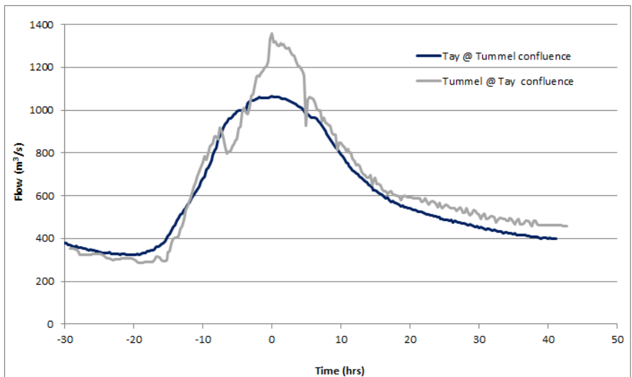
Diagram 4: Model III 0.5% AEP (200-year) inflow hydrograph in the Rivers Tay and Tummel for Run 1
