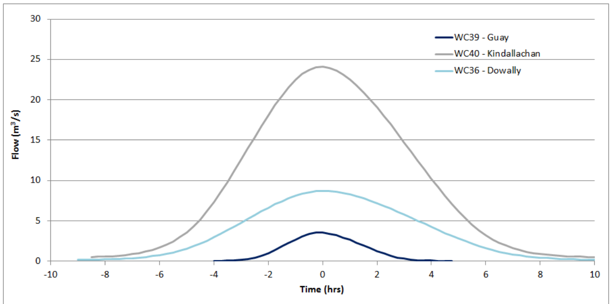
Diagram 6: Model III 0.5% (200-year) inflow hydrographs in the tributaries for Run 2
