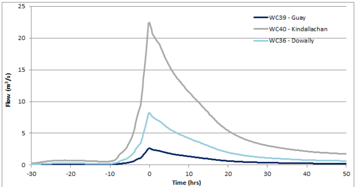
Diagram 6: Model III 0.5% (200-year) inflow hydrographs in the tributaries for Run 2
