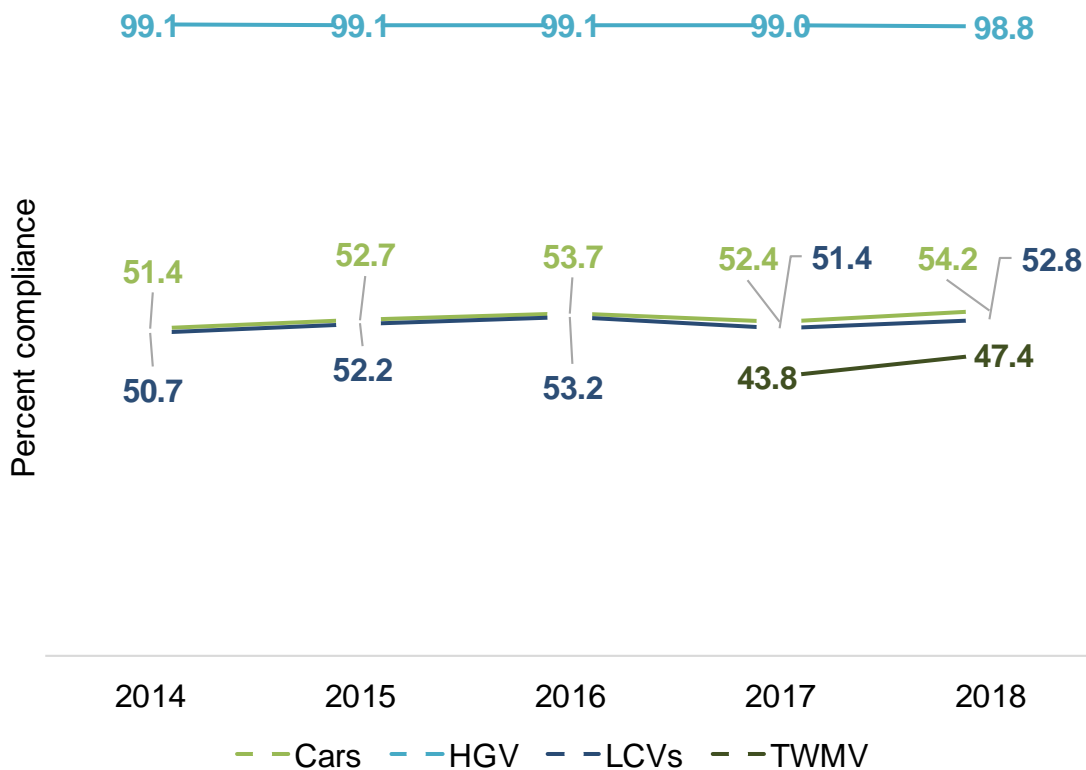
Figure 17 - Speed limit compliance by vehicle type – Motorways
