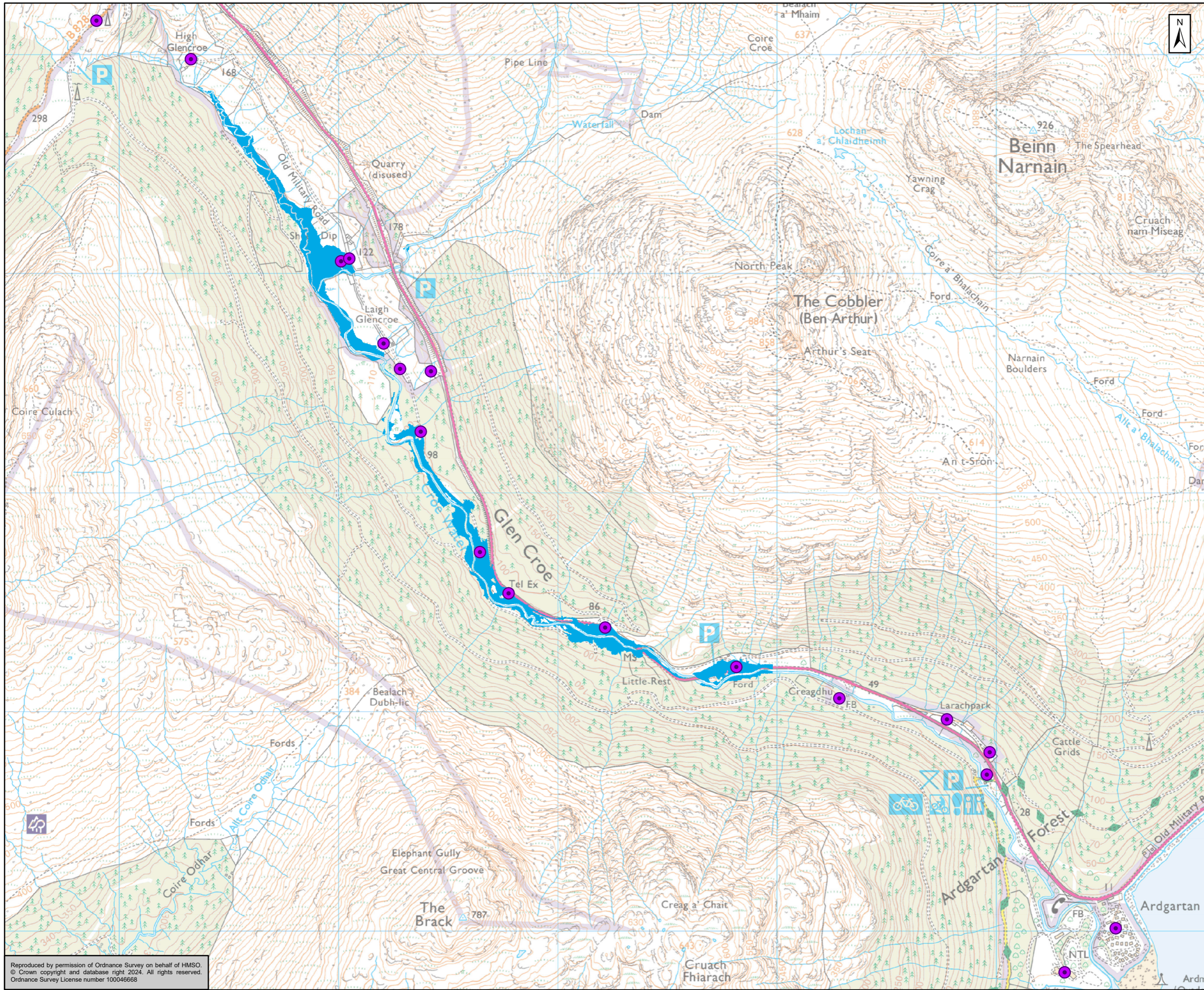
Figure 19.12 0.5%AEP +CC Max Flood Extent + Glen Croe sensitive receptors Page 1 of 1
