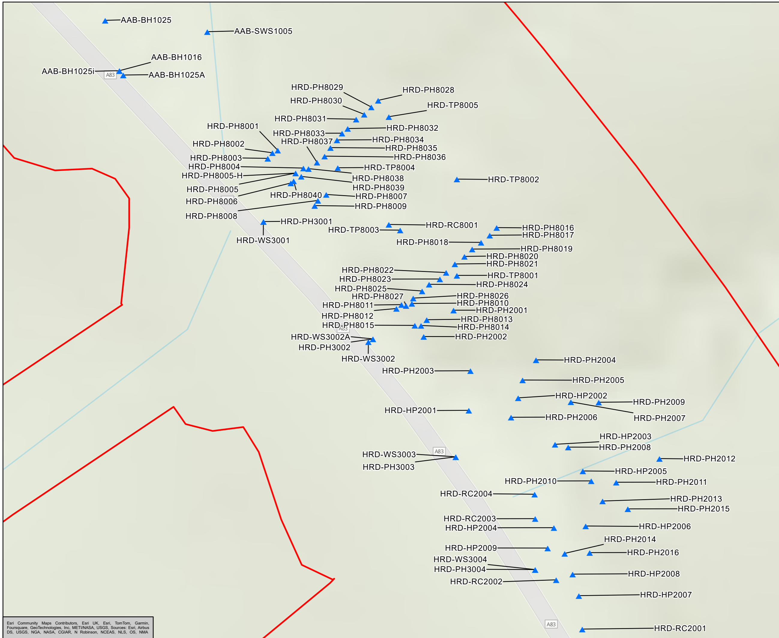
Figure 12.3 Ground Investigation Locations Page 5 of 7
