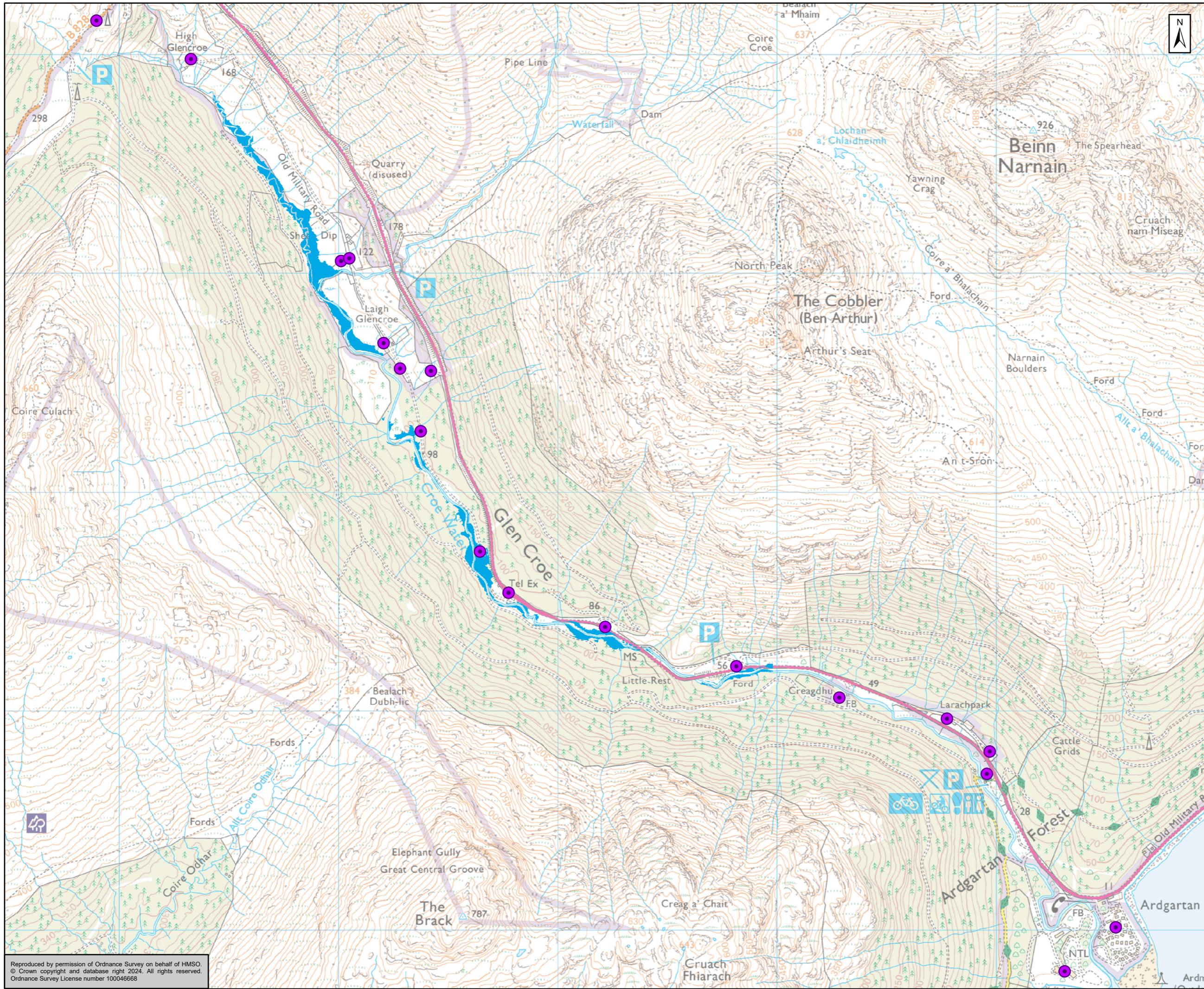
Figure 19.9 3.33%AEP Max Flood Extent + Glen Croe sensitive receptors Page 1 of 1
