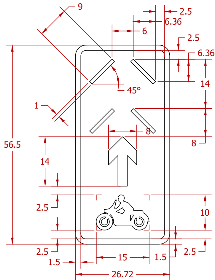
SIGN DIMENSIONS IN STROKE WIDTHS
