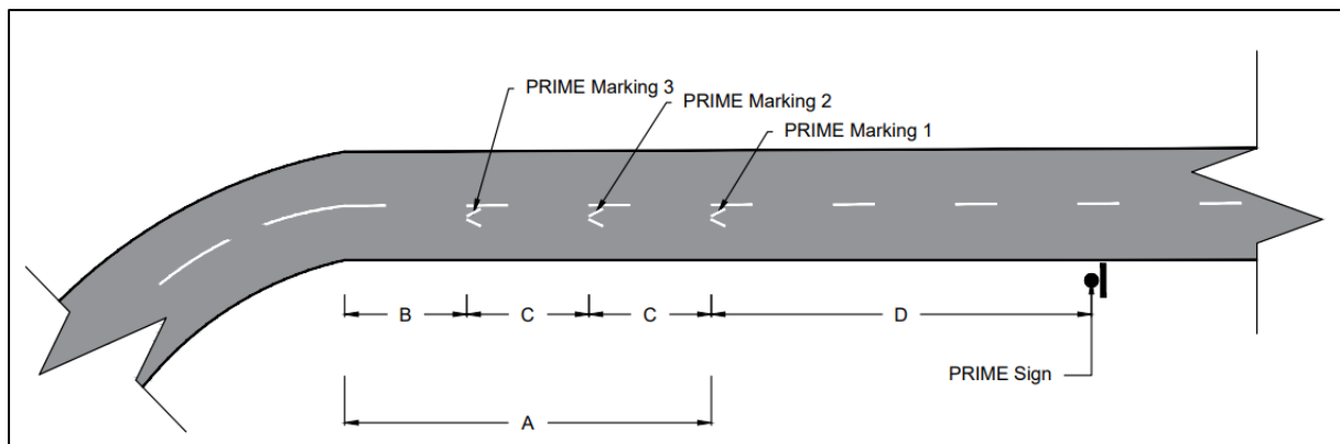
Figure 1: Setting out PRIME Road Markings and Signs
